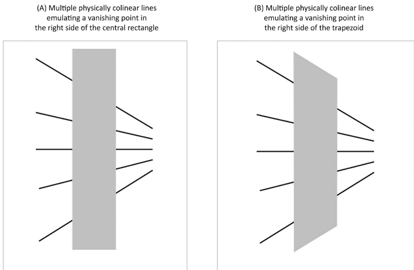
Figure 12. Poggendorff figures used to illustrate the possible effects of pictorial depth cues on the strength of the Poggendorff illusion. (A) Multiple physically collinear lines emulate a vanishing point on the right side of the rectangular central rectangle. (B) Multiple physically collinear lines emulate a vanishing point on the right side of the central trapezoid-like shape. Similar central areas were used by Gillam [11] to illustrate the effects of pictorial depth cues on the strength of the Poggendorff illusion. Gillam [11] demonstrated that the strength of the Poggendorff misalignment was weaker in Panel B and suggested that this was because it could be interpreted as a left-sidewall of a corridor.
