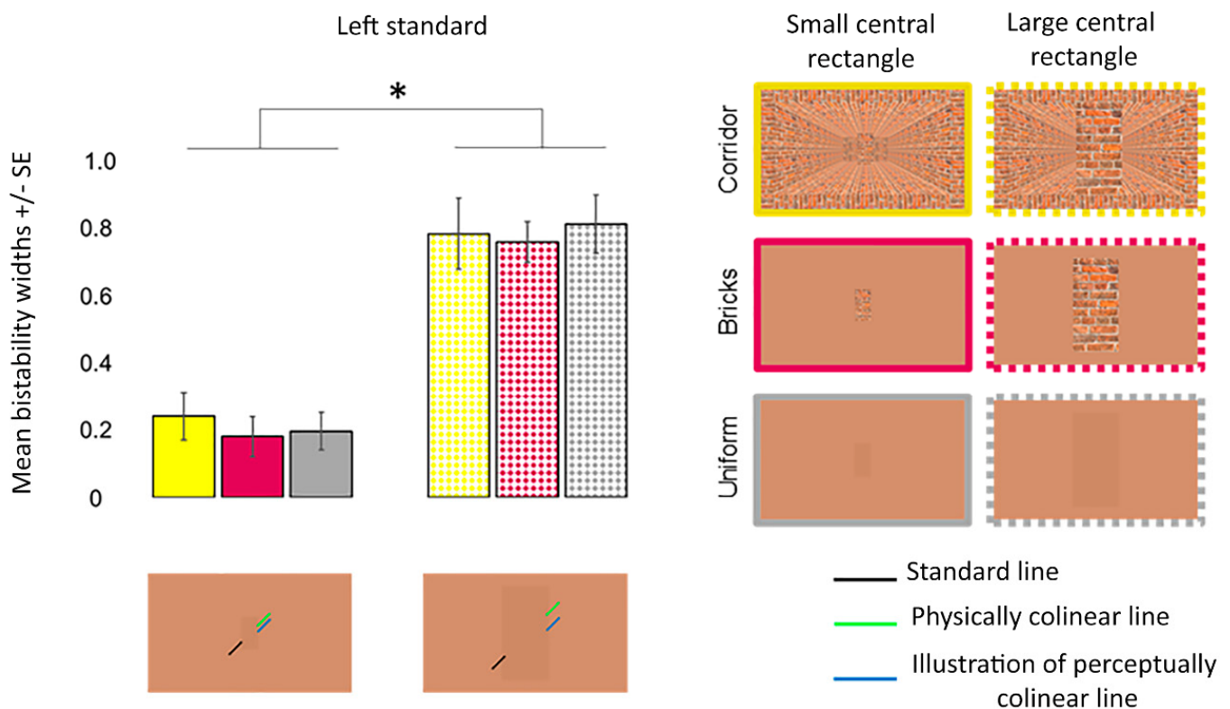
Figure 10. Mean bistability widths for the different conditions in experiment 3. The asterisk (*) denotes the difference between the perceptual uncertainty produced by the large and small central rectangles at p < 0.050 . Mean bistability widths were computed by subtracting P = 0.25 from P = 0.75 . Error bars denote standard errors for within-subject contrasts as described by O'Brien and Cousineau [22].
