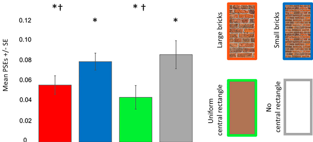
Figure 7. PSEs for the different Poggendorff stimuli in experiment 2. Daggers (†) denote differences from the no central rectangle condition at p < 0.050 after correcting for multiple comparisons using the Bonferroni method. Asterisks (*) denote differences from the physical width at p < 0.050 after correcting for multiple comparisons using the Bonferroni method. PSEs were computed from psychometric functions. Error bars denote standard errors for within-subject contrasts as described by O'Brien and Cousineau [22].
